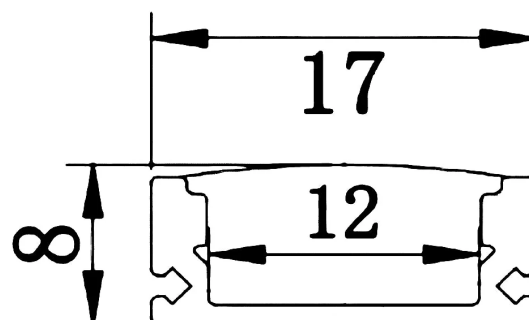
Cross-section — all dimensions in millimetres
