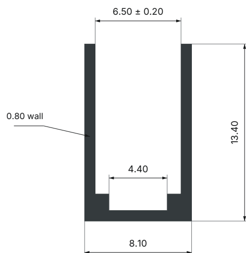
Cross-section in mm. Not to scale. Supplied drawing callouts; verify fit before installation.
