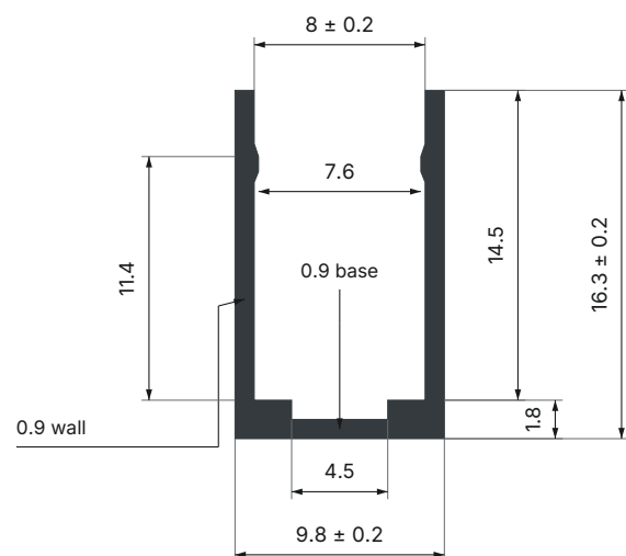
Cross-section in mm. Not to scale. Supplied drawing callouts; verify fit before installation.
