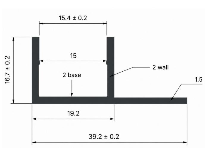
Cross-section in mm. Not to scale. Supplied drawing callouts; verify fit before installation.
