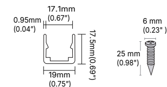
1 m Aluminum Channel
