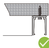
Correct: head clears neon.
