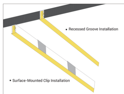
Flush / recessed
