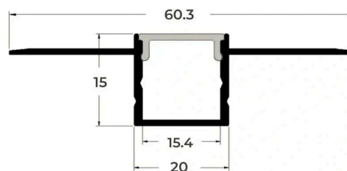
Cross-section — all dimensions in millimetres
