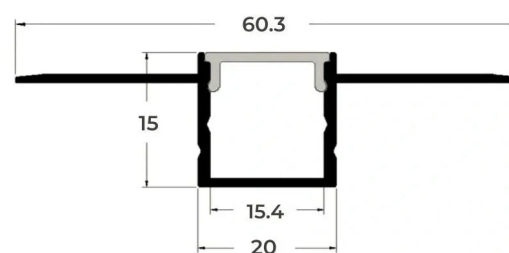
Cross-section — all dimensions in millimetres
