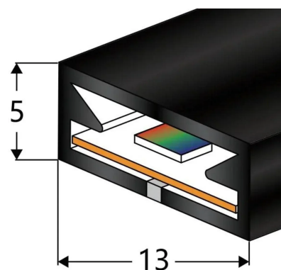
Cross-section — all dimensions in millimetres
