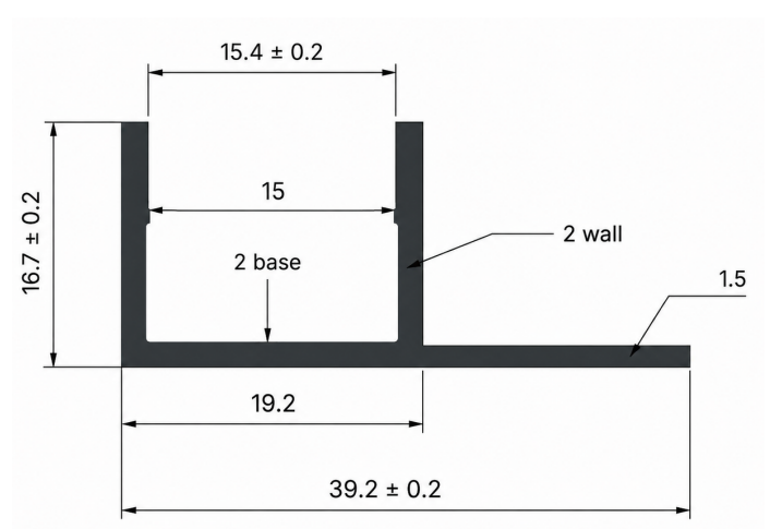
Cross-section in mm. Not to scale. Supplied drawing callouts; verify fit before installation.
