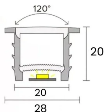
Cross-section — all dimensions in millimetres
