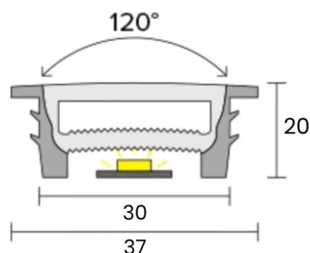
Cross-section — all dimensions in millimetres
