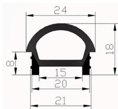
Cross-section — all dimensions in millimetres
